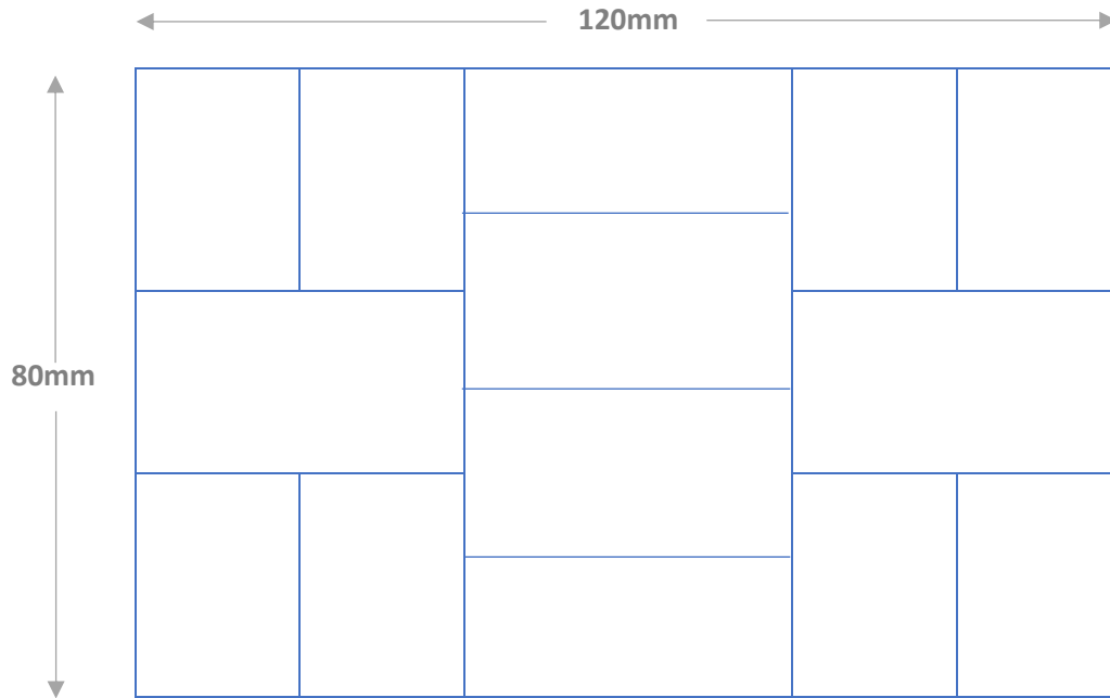
Pallet Configuration – Layers: 1, 4, 7
